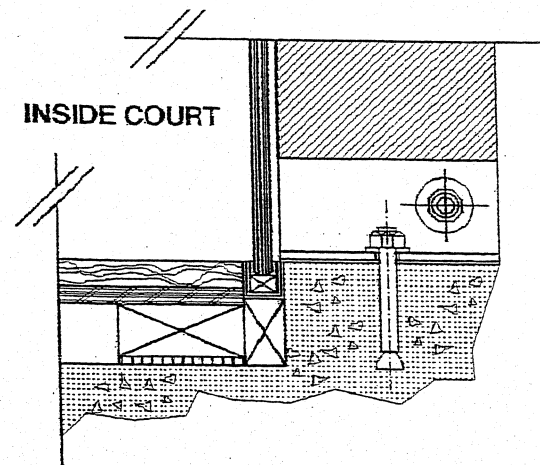
D-2 FLOOR/FIN DETAIL P-1 (STANDARD)
