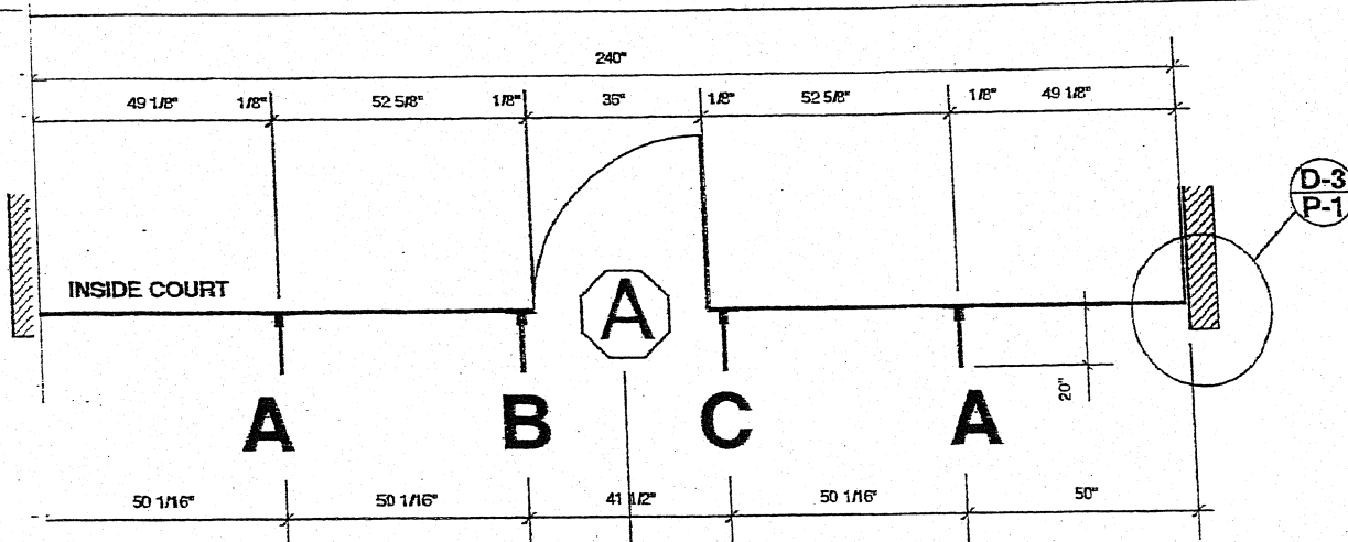
P PLAN: BACKWALL FIN LAYOUT P-1 Scale: 3/8" = 1'-0"
