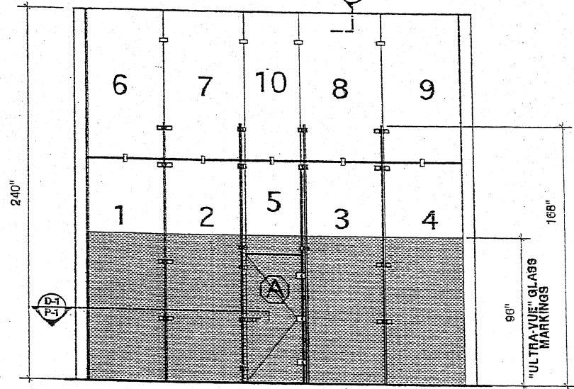
E-1 GLASS BACKWALL ELEVATION P-1 (View From Outside Of Court)
