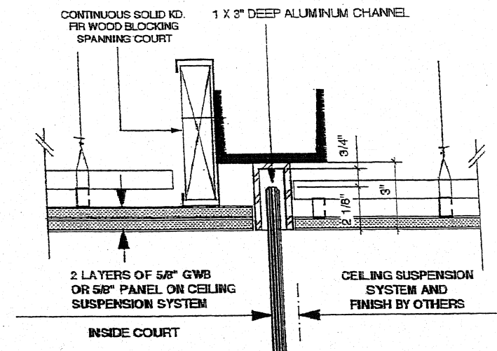
D-3 HEAD DETAIL P-1 TYPICAL
