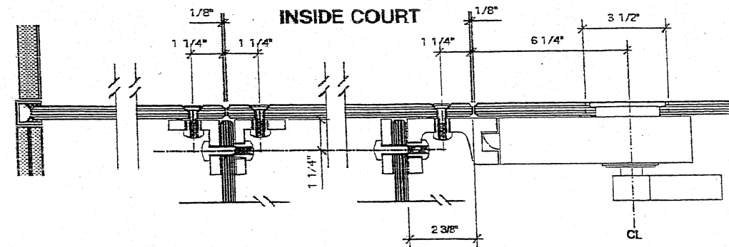
D-1 FIN/STRIKE/PASSAGE SET DETAIL P-1
