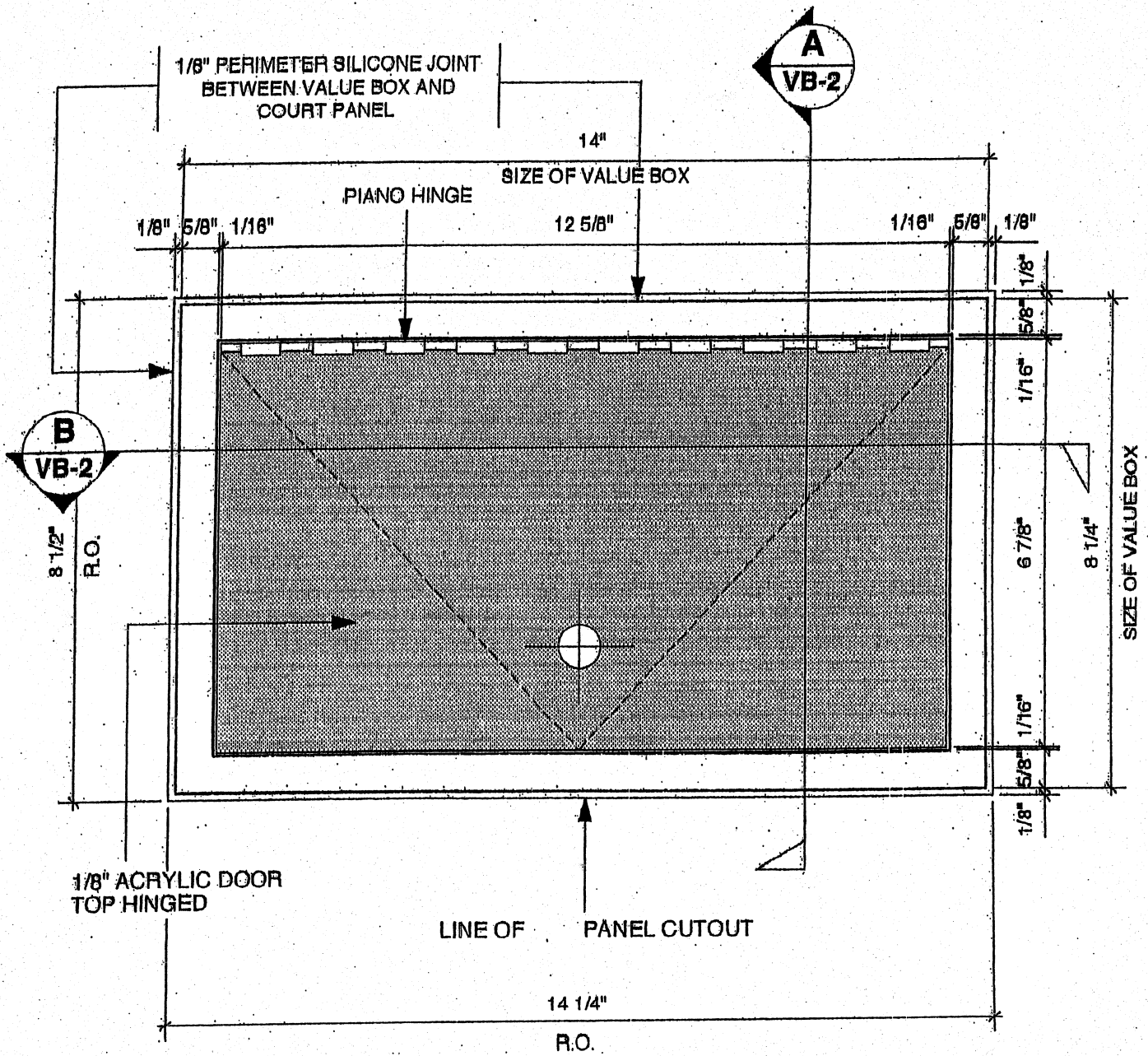
E-1 VB-1 ELEVATION VIEW FROM INSIDE COURT
